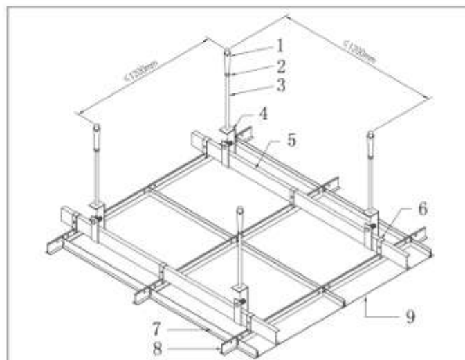
Lay-on Ceiling with T-bar System
