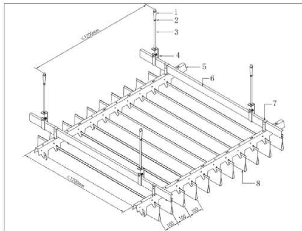
Dripping-baffle Ceiling System
