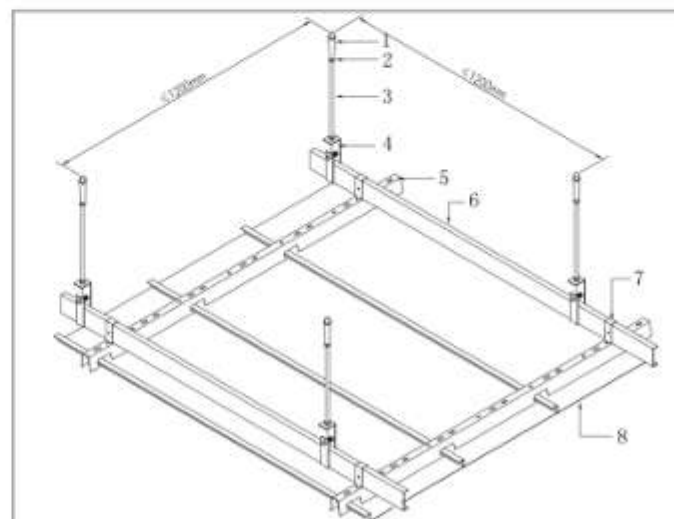
300/400/500H-strip Ceiling System
