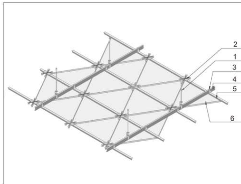
Triangular clip-in Ceiling System
