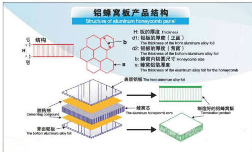
Structure of aluminum honeycomb panel
