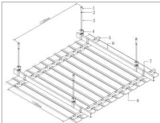
U-strip Ceiling System
