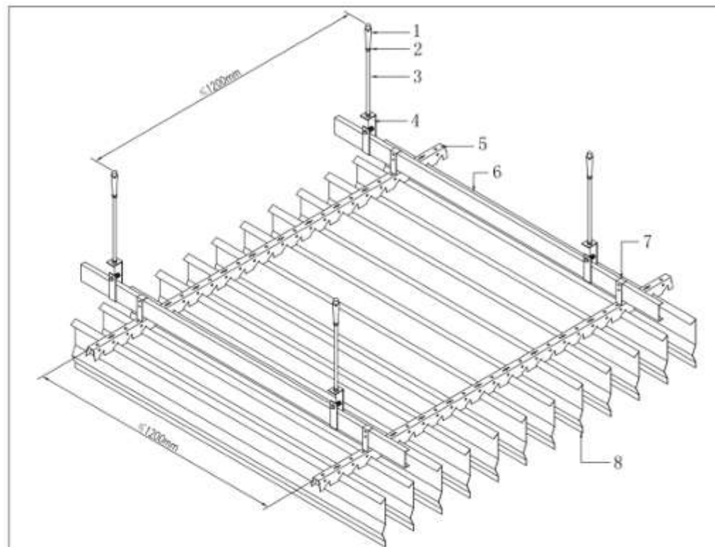
A-screen Ceiling System
