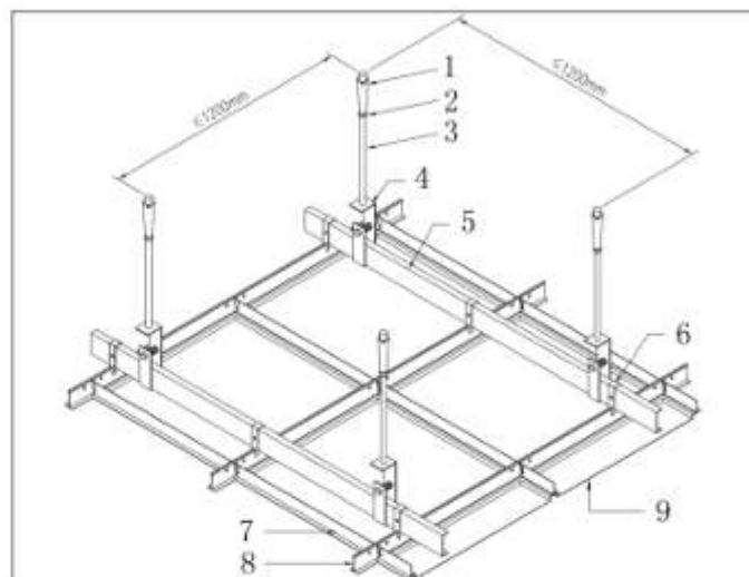
Lay-in Ceiling with T-bar System
