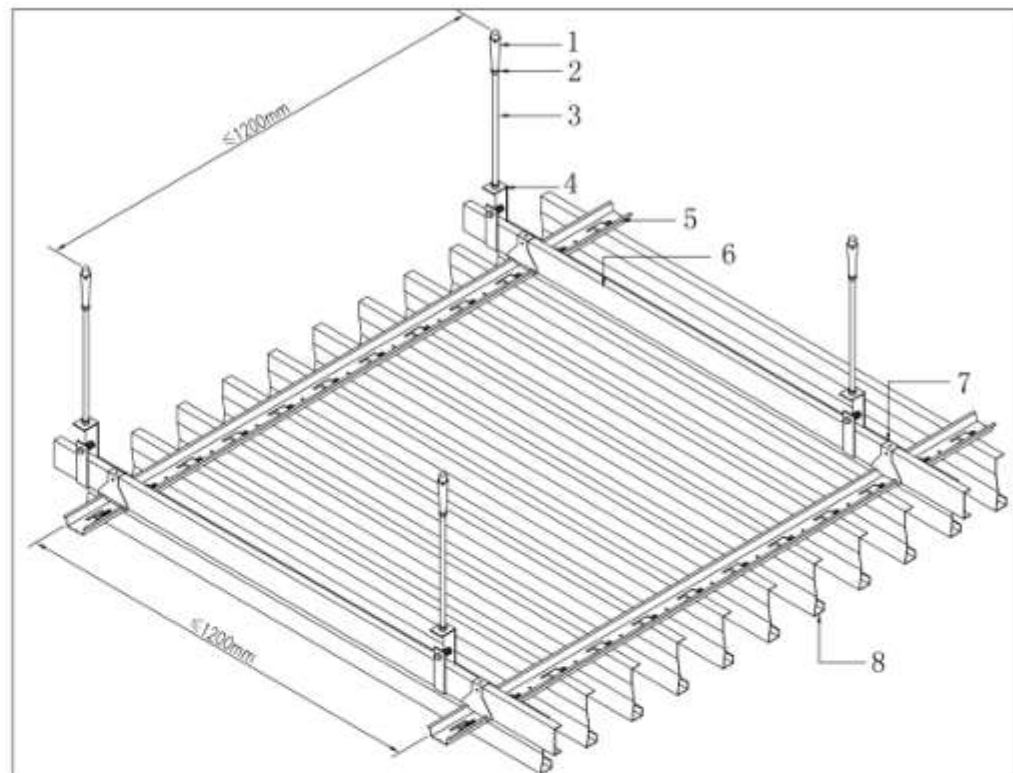
E-screen Ceiling System
