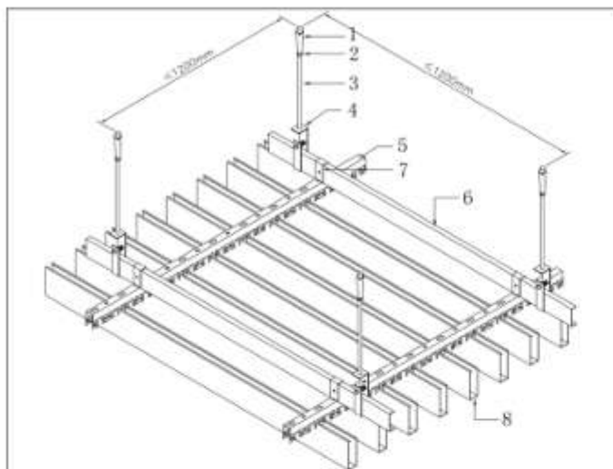
U-baffle Ceiling System
