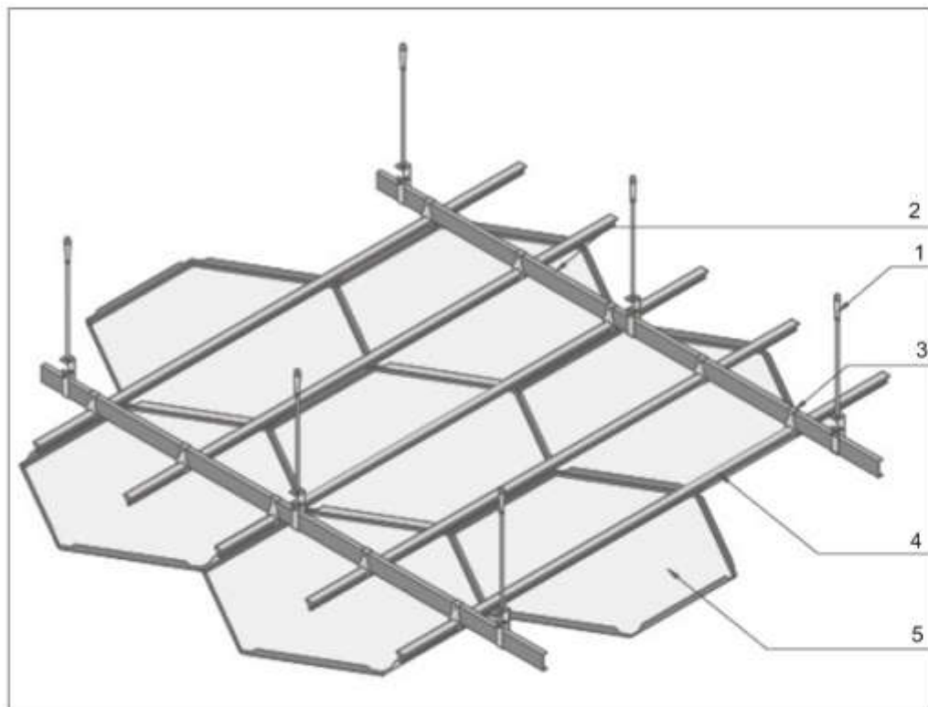
Hexagonal clip-in Ceiling System
