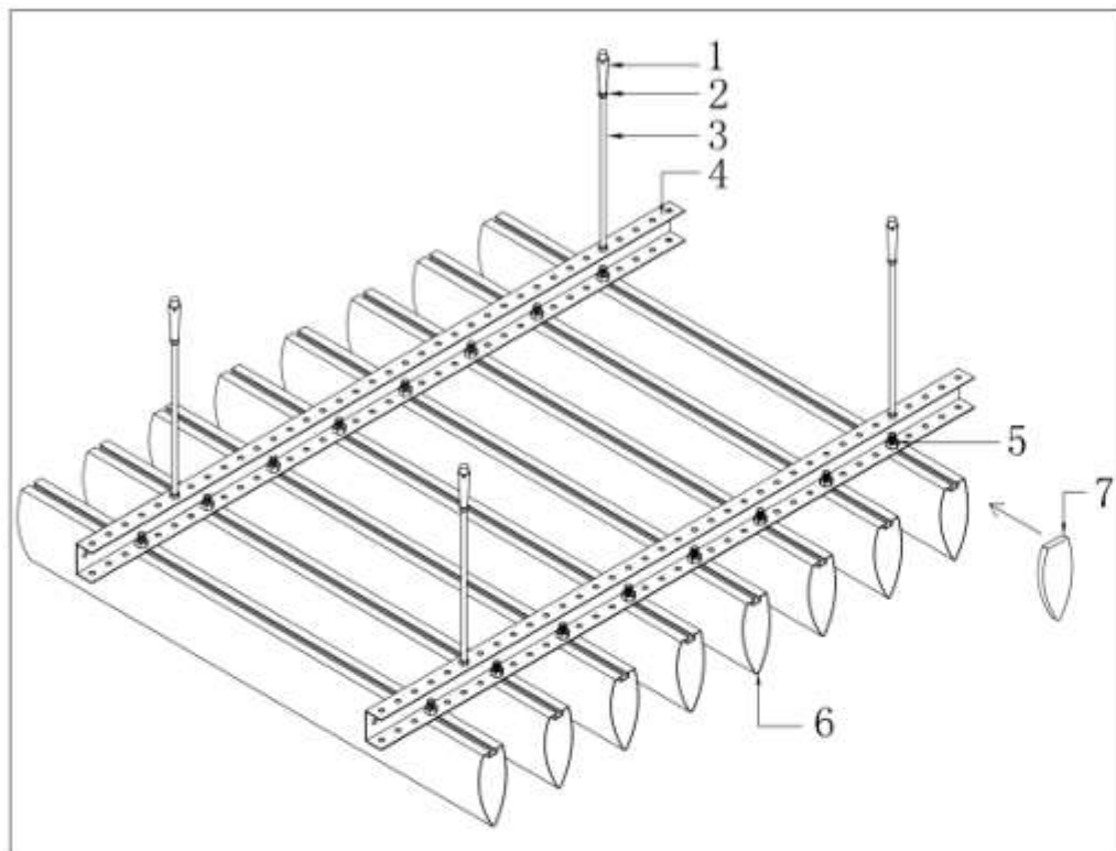
Bullet-baffle Ceiling System
