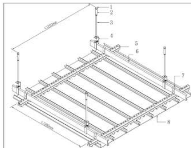
Square edge S-strip Ceiling System
