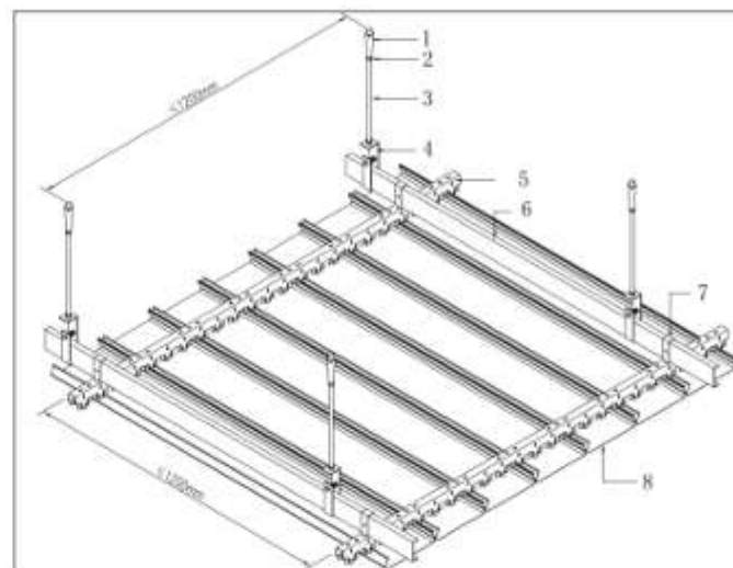
Bevelled edge S-strip Ceiling System
