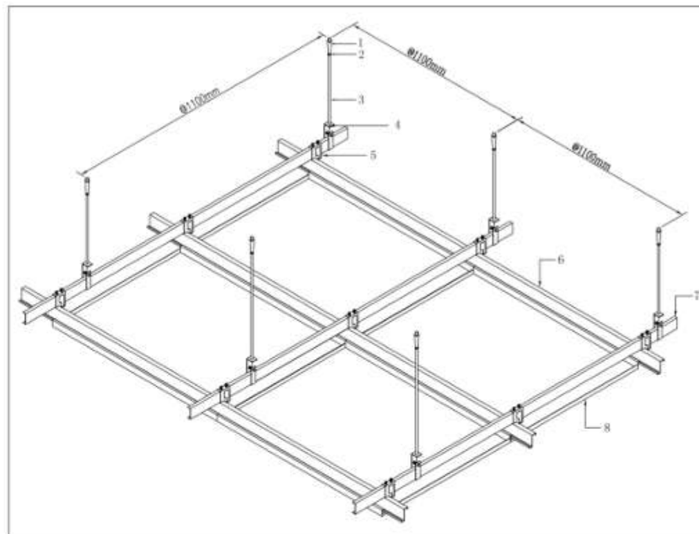
Hook-on Ceiling System
