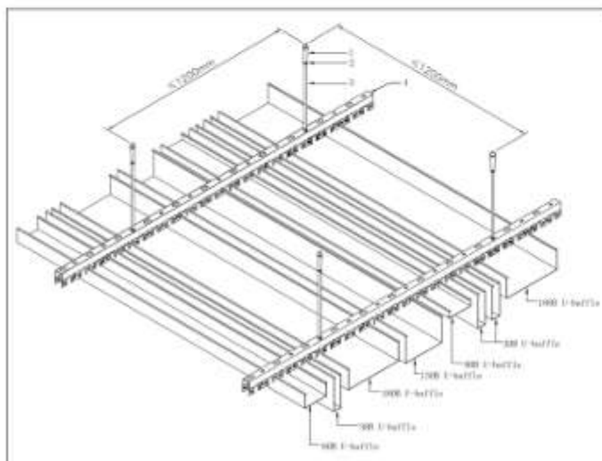
Multi U-baffle Ceiling System
