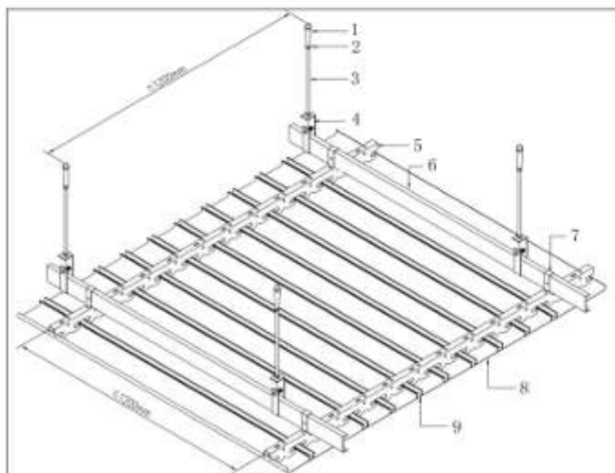
U-strip with infilled Ceiling System
