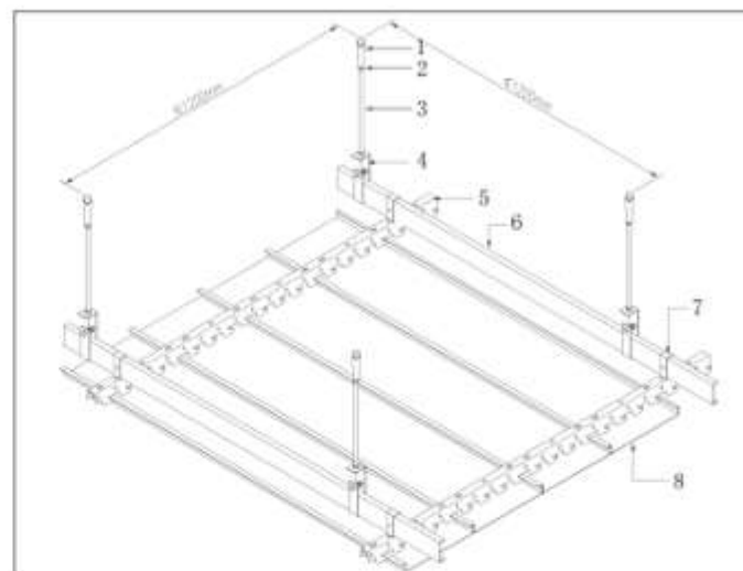
150/200H-strip Ceiling System
